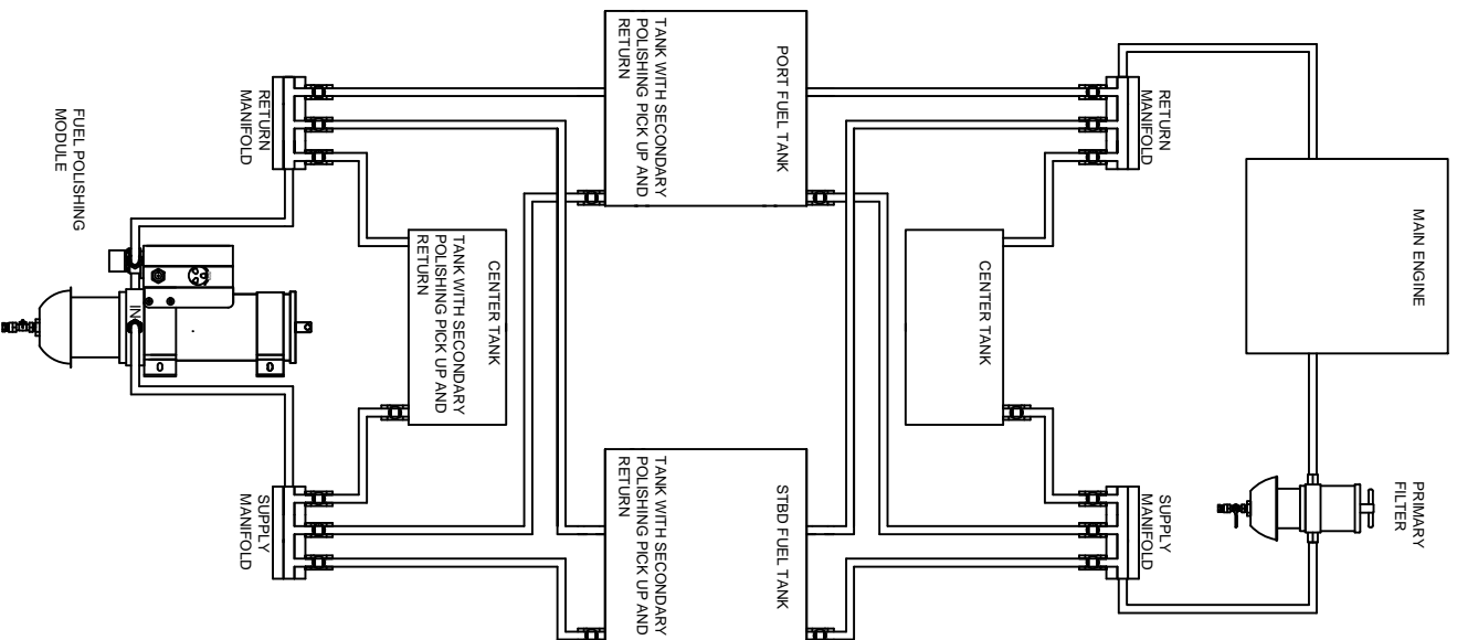
MULTI TANK - FPM USING A SEPARATE SUPPLY AND RETURN MANIFOLD
